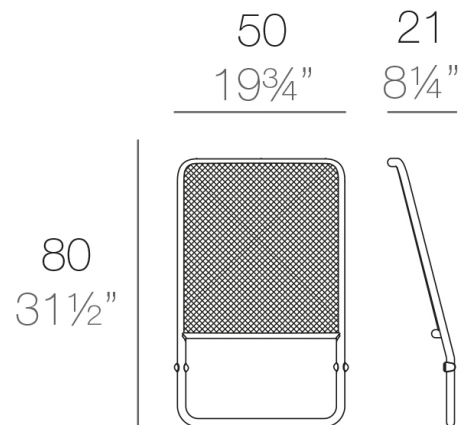
KES Respaldo Alto KES High Backrest
