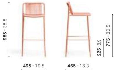
3668 Barstool, steel frame, PVC flexible profile seat and backrest
