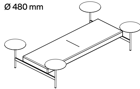
Nia wall L 2400/2860 P 600/1100 H 400/602 mm Ø 480 mm
